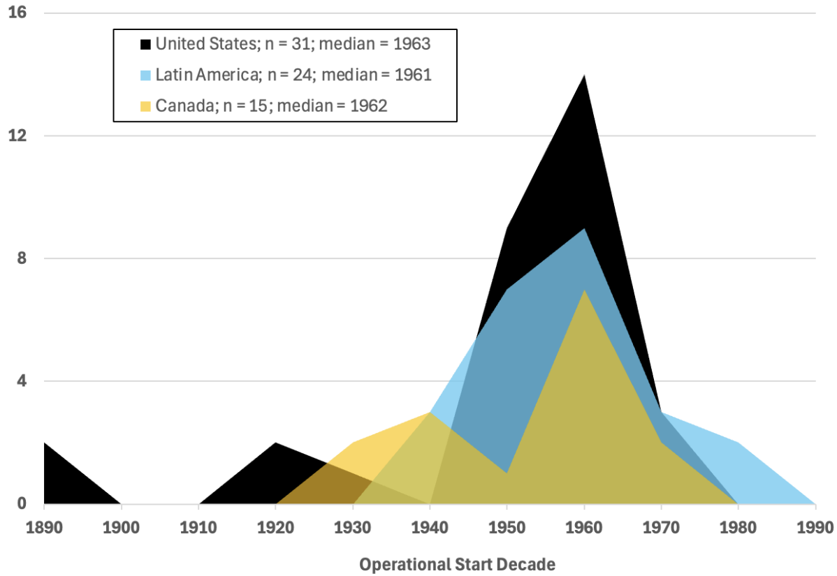
Temporal Distribution - Mercury Cell Chlor-Alkali Construction in the Americas
